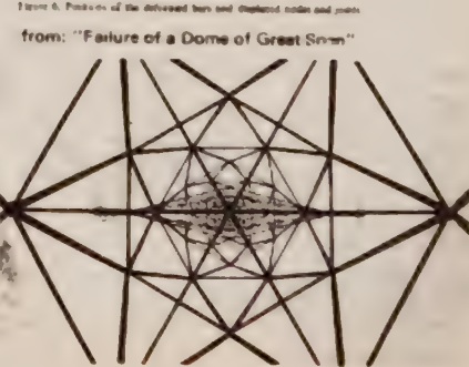
Figure 2. View looking up and from the center of the dome.
